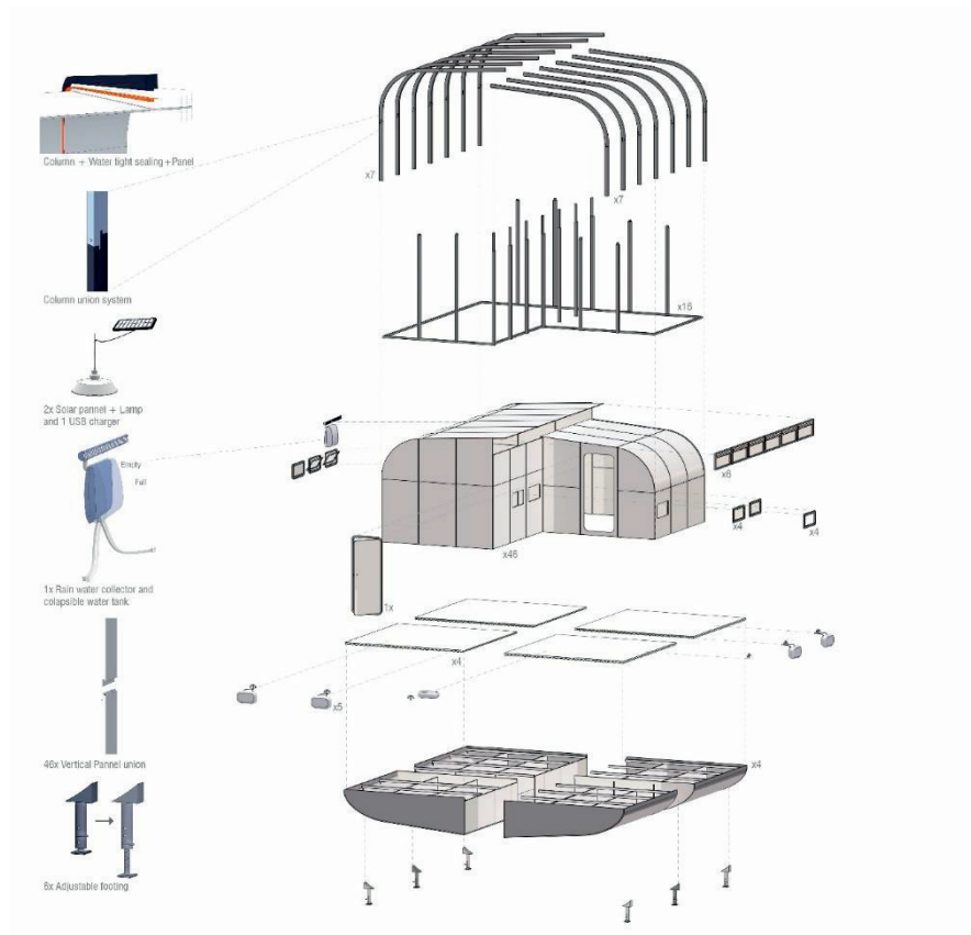
Figure 9. Exploded axonometric view.
