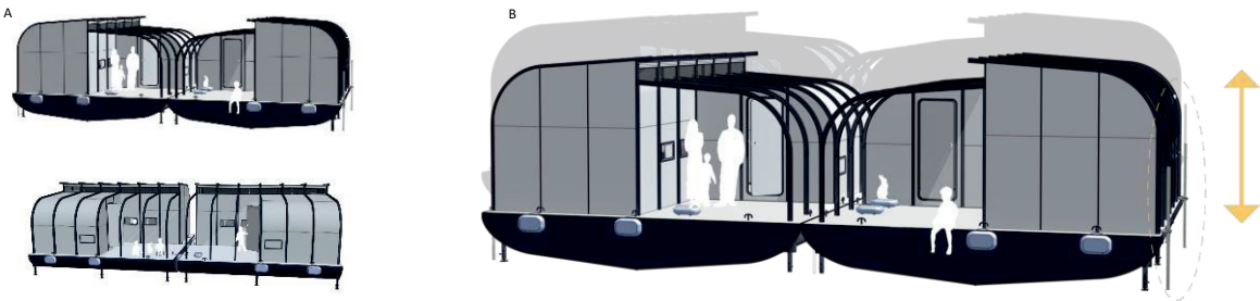
Figure7. Shelter arrangements for large families (A). Vertical movement of the shelter when used as amphibious option, fixed to the ground by its lateral guide poles (B).
