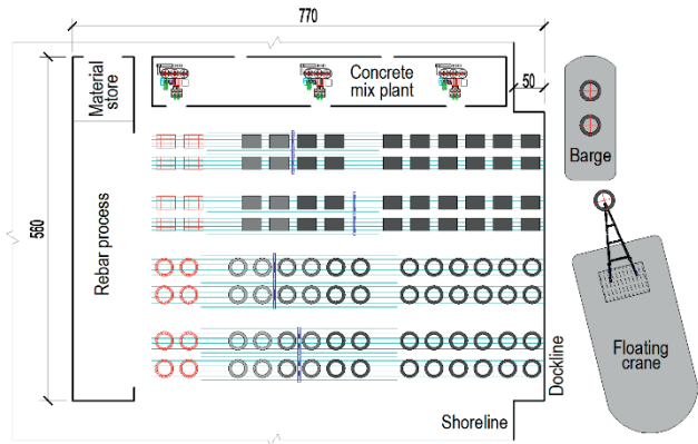
(b) factory conceptual layout for mega shelter
