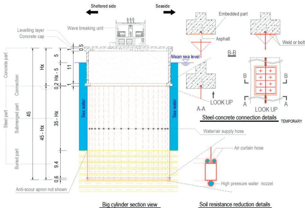
(a) details including temporary installation facilities
