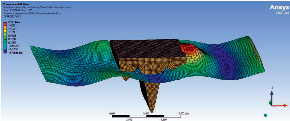
Fig. 5: 3D view of a trident shape with wave loading
